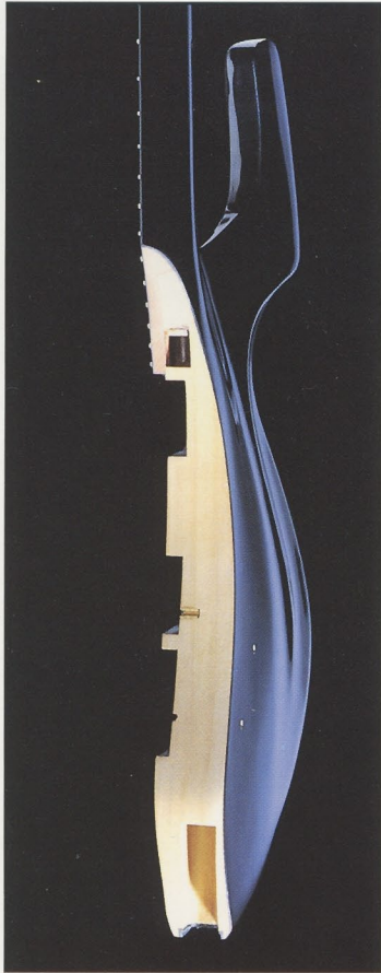
Cut-away of Parker Fly Deluxe
